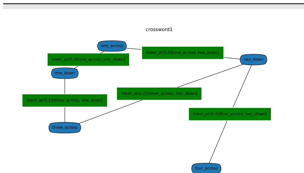
Figure 4.6: crossword1.show()
