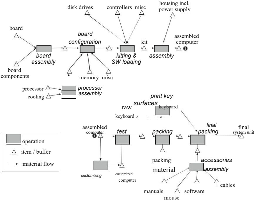
Fig. 23.2 Detailed computer assembly supply chain
