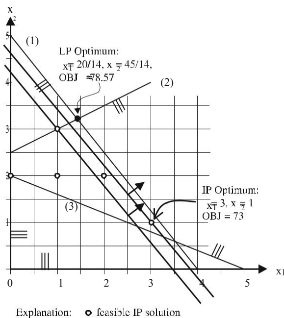
Fig. 30.4 A graphical representation of an IP model
