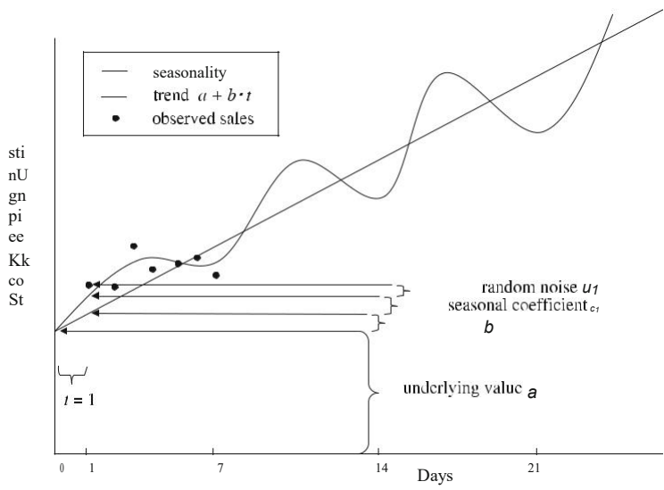
Fig. 29.2 Modeling seasonality and trend
