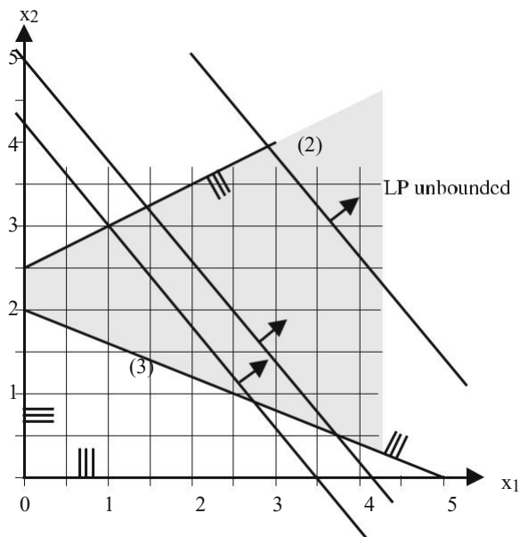
Fig. 30.3 An unbounded LP model
