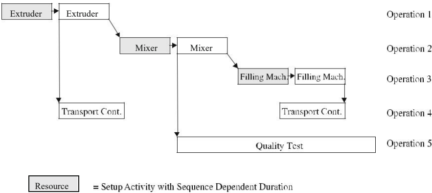
Fig. 22.3 PPM structure of the production process
