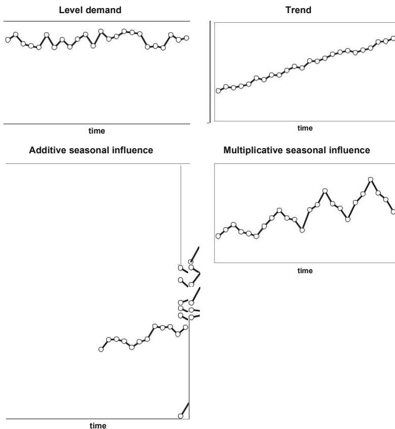
Fig. 7.8 Demand patterns
