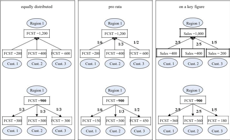
Fig. 20.5 Disaggregation rules
