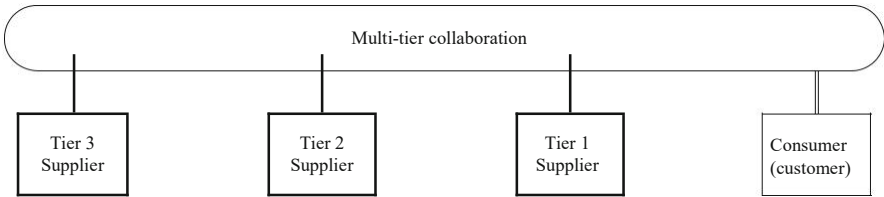
Fig. 14.5 Multi-tier collaboration
