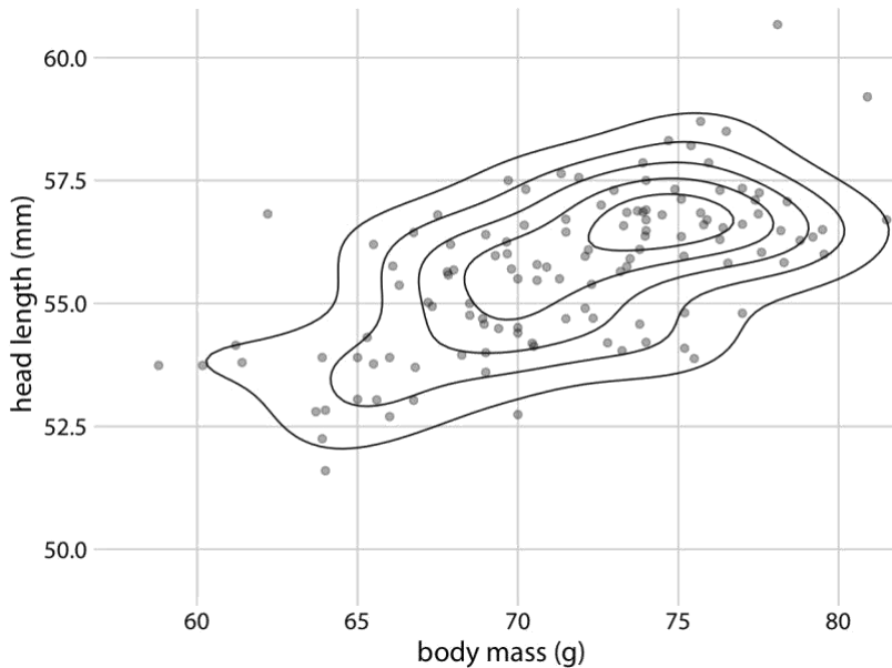
Figure 18-8. Head length versus body mass for 123 blue jays, as in Figure 12-1 . Each dot corresponds to one bird, and the lines indicate regions of similar point density. The point density increases toward the center of the plot, near a body mass of 75 g and a head length between 55 mm and 57.5 mm. Data source: Keith Tarvin, Oberlin College.
