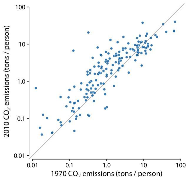
Figure 12-11. Carbon dioxide emissions per person in 1970 and 2010, for 166 countries. Each dot represents one country. The diagonal line represents identical CO 2 emissions in 1970 and 2010. The points are systematically shifted upwards relative to the diagonal line: in the majority of countries, emissions were higher in 2010 than in 1970. Data source: Carbon Dioxide Information Analysis Center.
