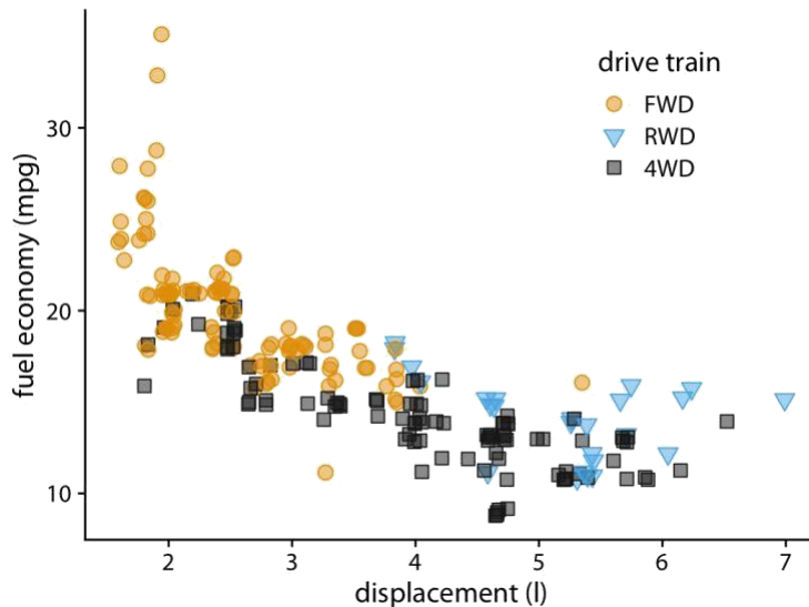
Figure 25-7. City fuel economy versus engine displacement. By using both different col- ors and different solid shapes for the different drive-train variants, this figure visually separates the drive-train variants while remaining reproducible in grayscale if needed. Data source: EPA.
