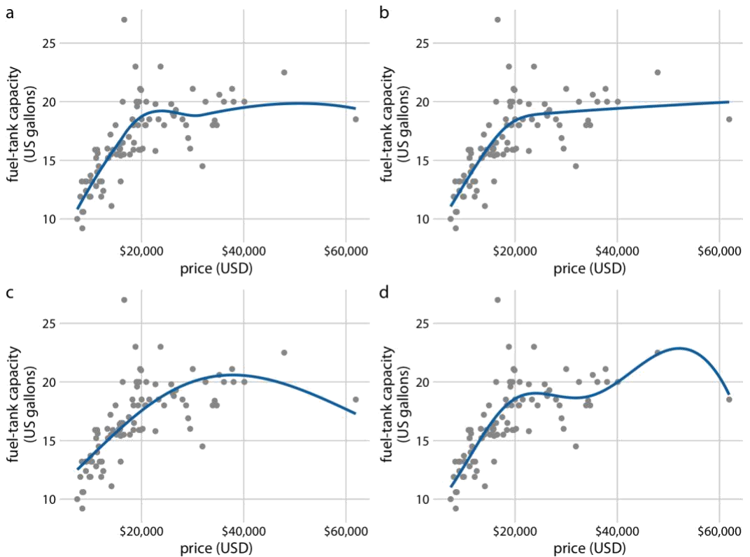
Figure 14-5. Different smoothing models display widely different behaviors, in particular near the boundaries of the data. (a) LOESS smoother, as in Figure 14-4 . (b) Cubic regression splines with 5 knots. (c) Thin-plate regression spline with 3 knots. (d) Gaussian process spline with 6 knots. Data source: Robin H. Lock, St. Lawrence University.
