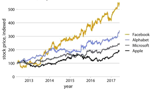
tritanomaly
