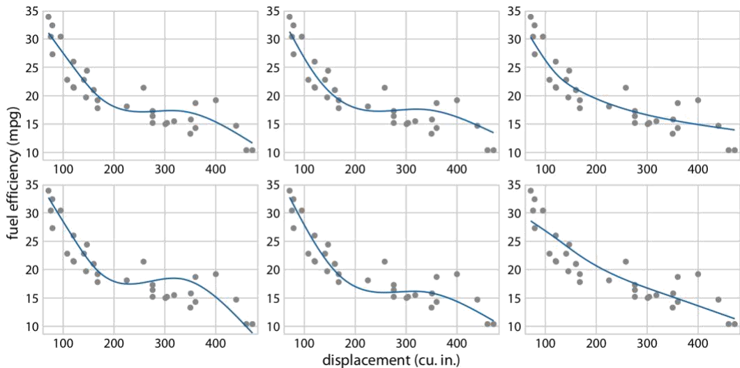
Figure 16-20. Schematic of a hypothetical outcome plot for fuel efficiency versus displacement. Each dot represents one car, and the smooth lines were obtained by fitting a cubic regression spline with 5 knots. Each line in each panel represents one alternative fit outcome, drawn from the posterior distribution of the fit parameters. In an actual hypothetical outcome plot, the display would cycle between the distinct plot panels instead of showing them side-by-side. Data source: Motor Trend, 1974.
