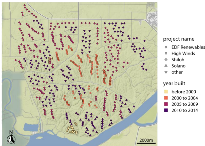
Figure 15-10. Locations of individual wind turbines in the Shiloh Wind Farm. Each dot highlights the location of one wind turbine. The map area corresponds to the top rectangle in Figure 15-8. Dots are colored by when the wind turbine was built, and the dot's shape represents the project to which an individual wind turbine belongs. Map tiles by Stamen Design, under CC BY 3.0. Map data by OpenStreetMap, under ODbL. Wind turbine data source: US Wind Turbine Database.
