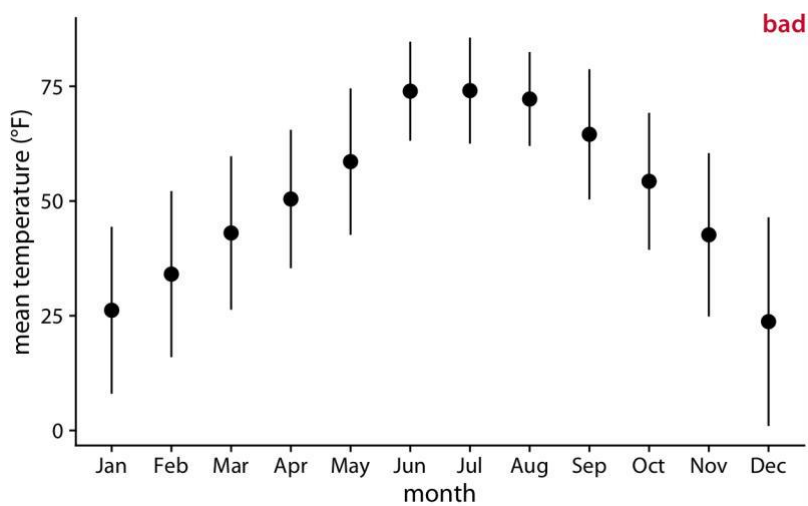
Figure 9-1. Mean daily temperatures in Lincoln, NE, in 2016. Points represent the average daily mean temperatures for each month, averaged over all days of the month, and error bars represent twice the standard deviation of the daily mean temperatures within each month. This figure has been labeled as “bad” because error bars are conventionally used to visualize the uncertainty of an estimate, not the variability in a population. Data source: Weather Underground.
