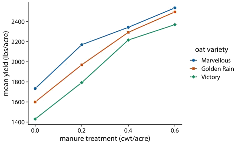
Figure 13-8. Dose-response curve showing the mean yield of oat varieties after fertilization with manure. The manure serves as a source of nitrogen, and oat yields generally increase as more nitrogen is available, regardless of variety. Here, manure application is measured in cwt (hundredweight) per acre. The hundredweight is an old imperial unit equal to 112 lbs or 50.8 kg. Data source: [Yates 1935].
