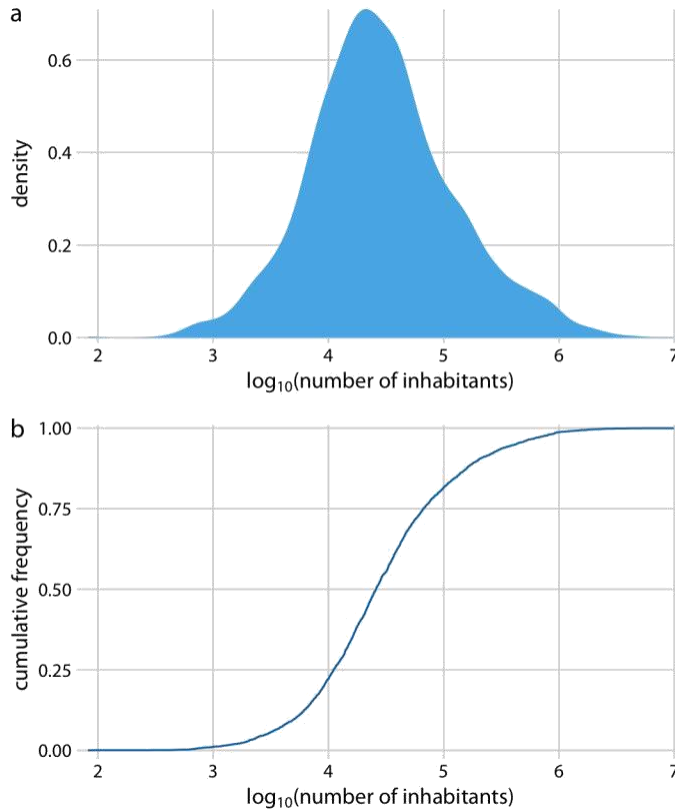
Figure 8-5. Distribution of the logarithm of the number of inhabitants in US counties. (a) Density plot. (b) Empirical cumulative distribution function. Data source: 2010 US Decennial Census.
