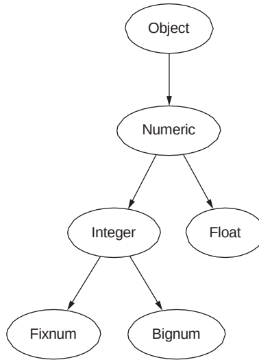
FIG. 5.2 A class hierarchy, described by the number.dot file and converted to a visual file, using GraphViz.
