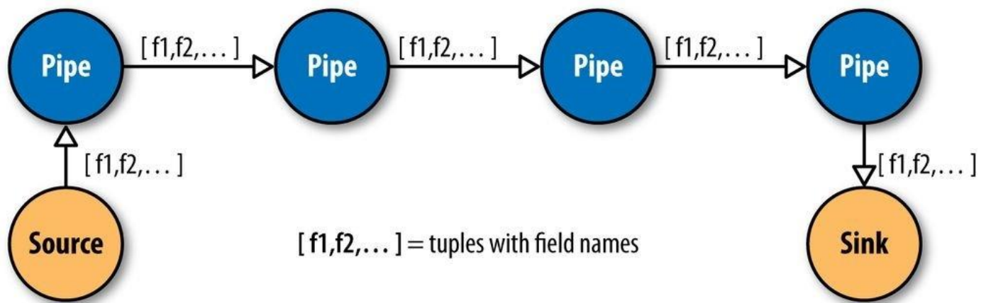
Figure 24-2. Pipes linked by fields and tuples
