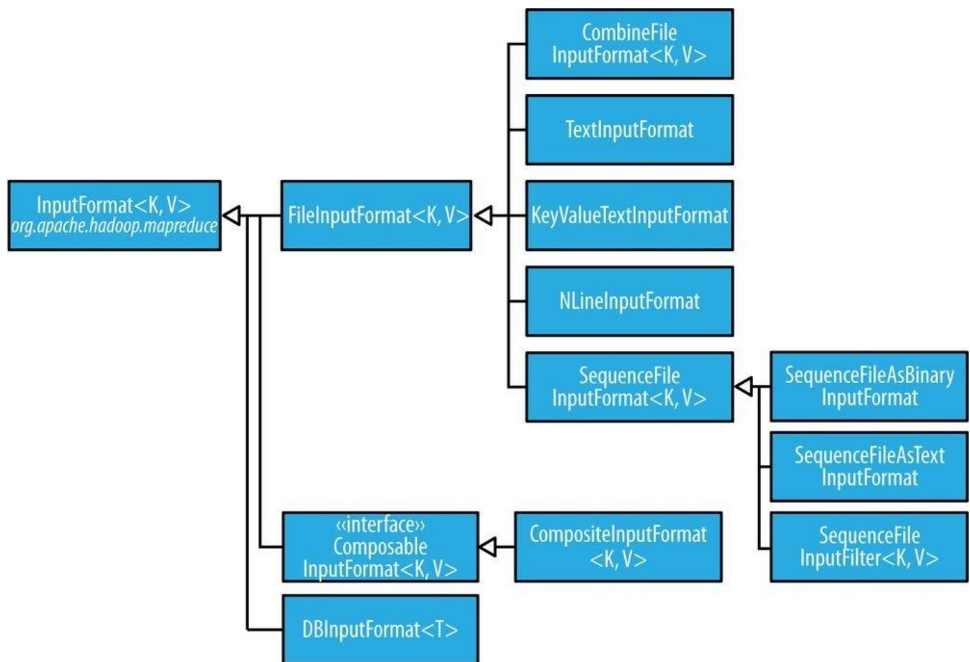
Figure 8-2. InputFormat class hierarchy
