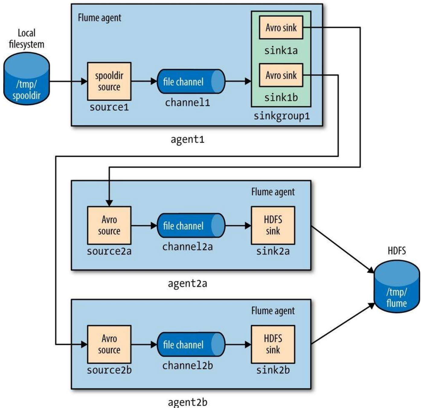
Figure 14-6. Load balancing between two agents
