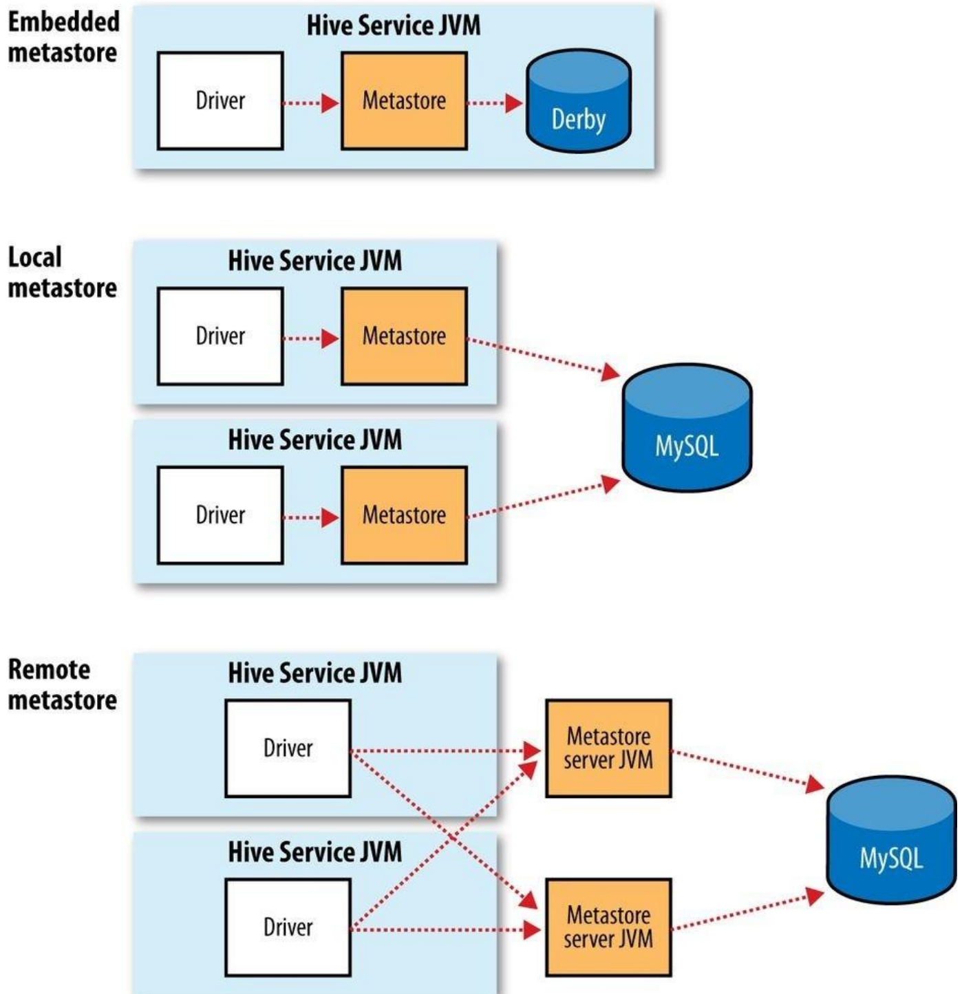
Figure 17-2. Metastore configurations
