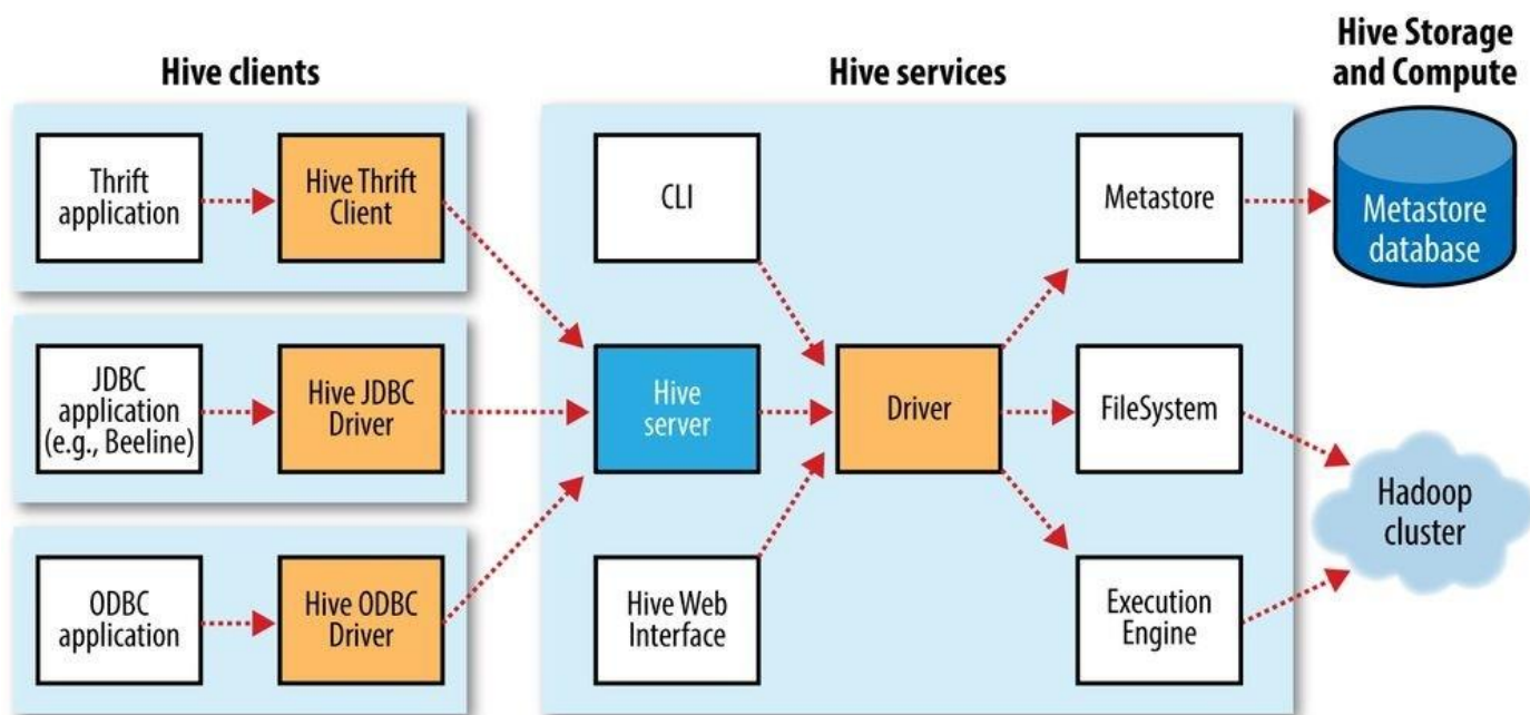
Figure 17-1. Hive architecture
