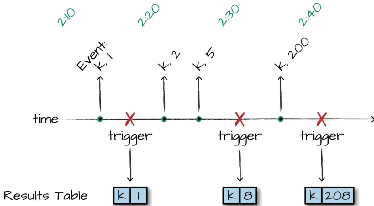
Figure 22-3. Sliding Windows
