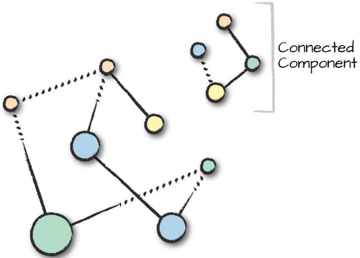
Figure 30-5. A connected component
