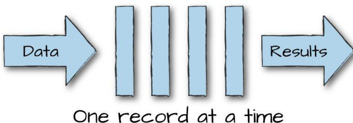
Figure 20-1. Continuous processing
