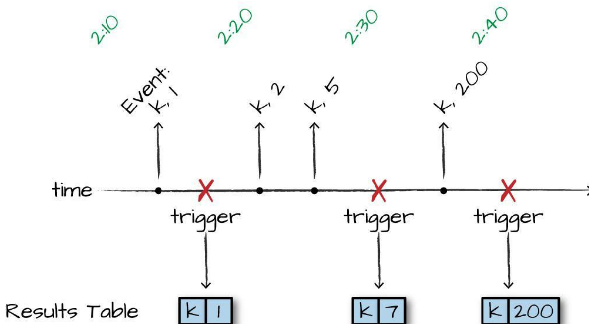
Figure 22-2. Tumbling Windows
