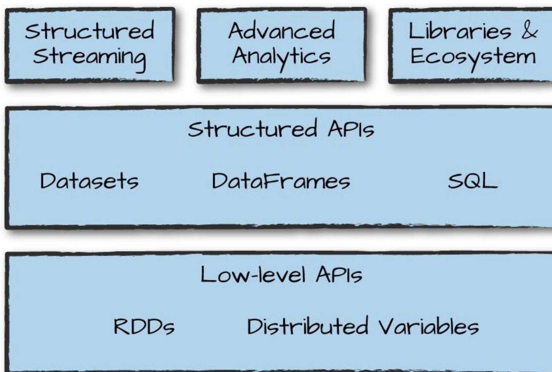
Figure 1-1. Spark's toolkit
