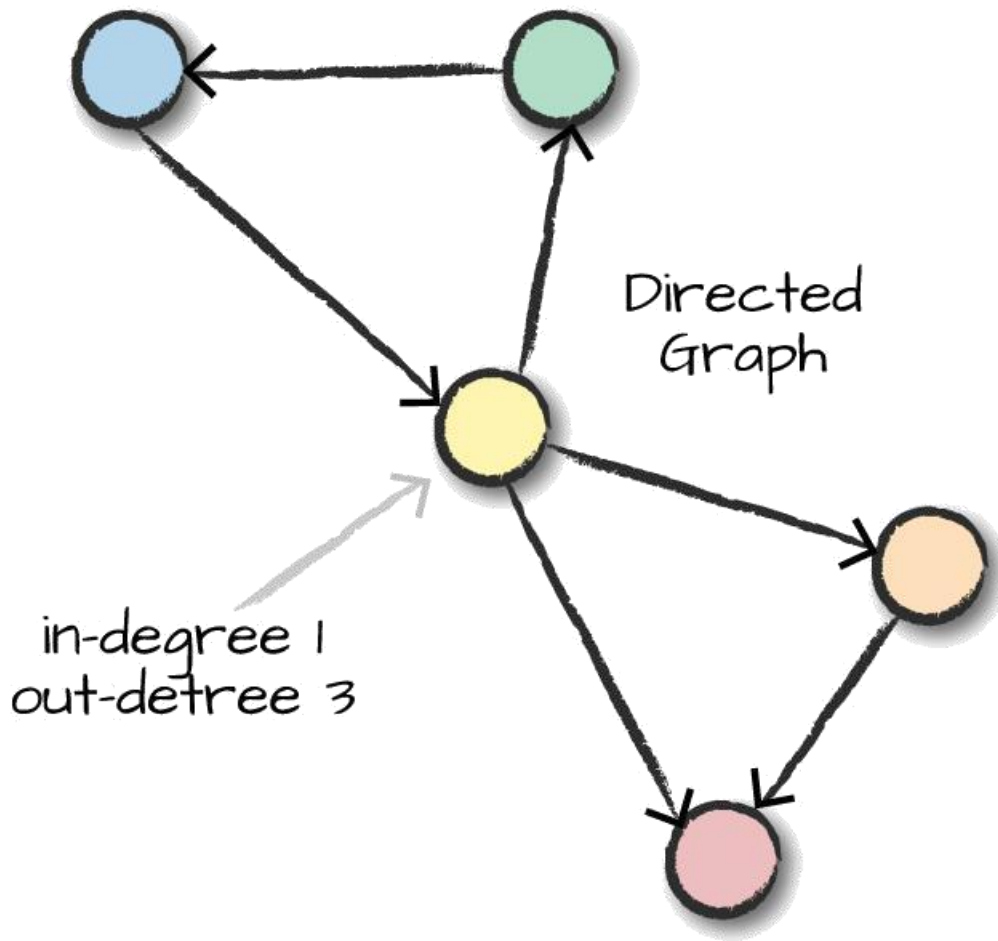
Figure 30-4. In-degree and out-degree
