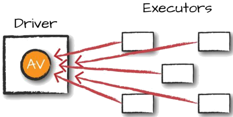
Figure 14-2. Accumulator variable
