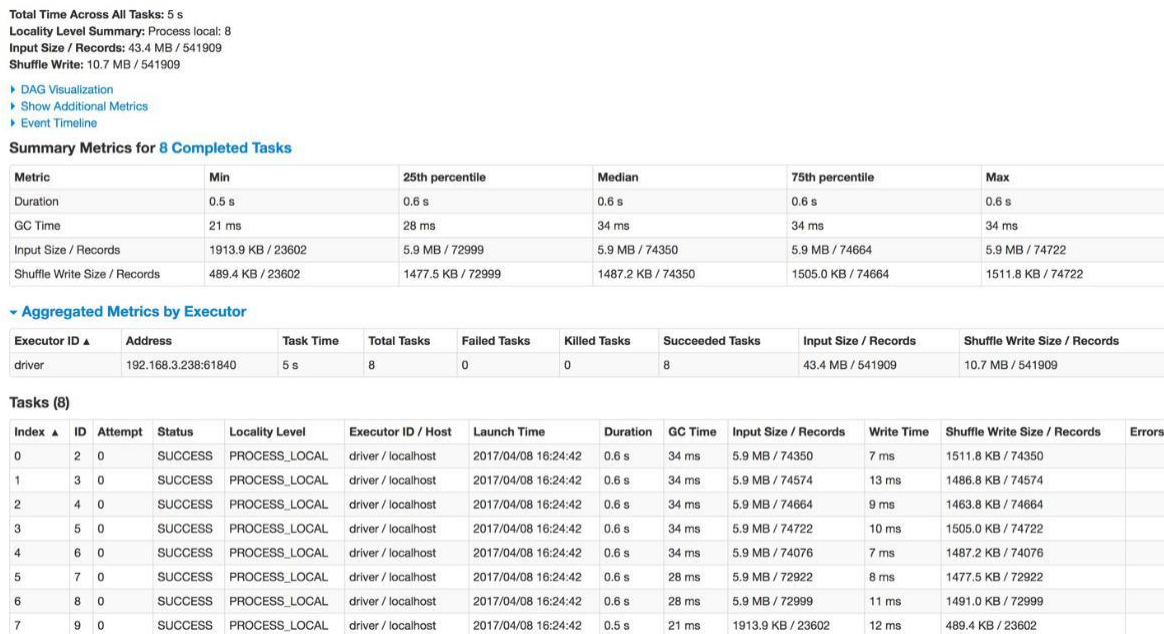
Figure 18-8. Spark tasks
