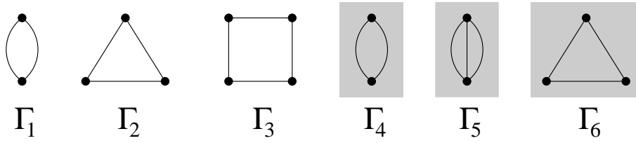
Figure 3.16: Some regular cell complexes
