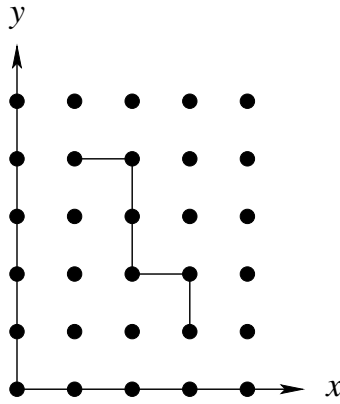
Figure 2.4: A lattice path in \mathbb{N}^2
