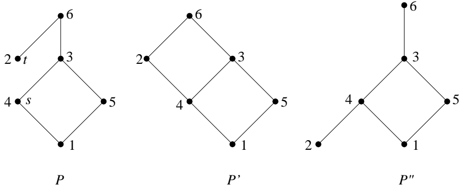
Figure 3.58: The procedure P \rightarrow (P', P'')
