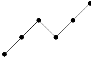
Figure 3.68: A solution to Exercise 3.7
