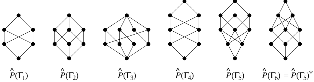
Figure 3.17: The face posets of the regular cell complexes of Figure 3.16
