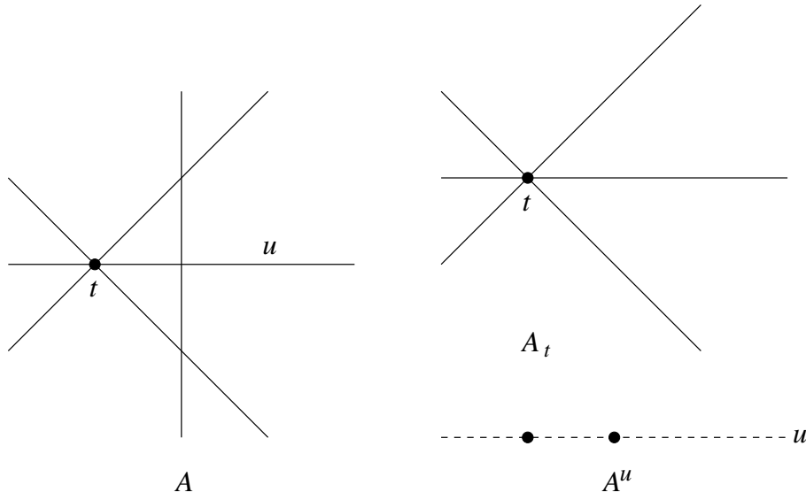
Figure 3.21: An illustration of the definitions of \mathcal{A}_t and \mathcal{A}^u
