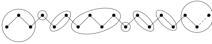
Figure 3.75: Illustration of the solution to Exercise 3.66(d)
