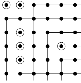
Figure 1.5: The diagram of the permutation w = 314652
