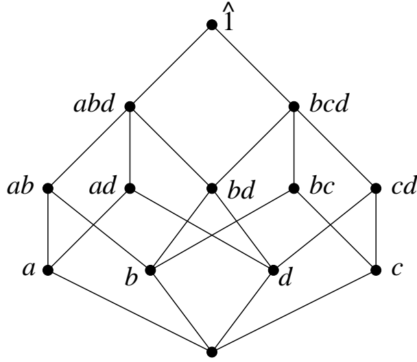
Figure 4.5: Face poset of the triangulation of Figure 4.4
