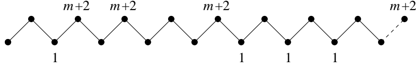
Figure 3.76: Continuing the solution to Exercise 3.66(d)
