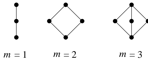
Figure 3.19: Face posets of some 0-dimensional manifolds
