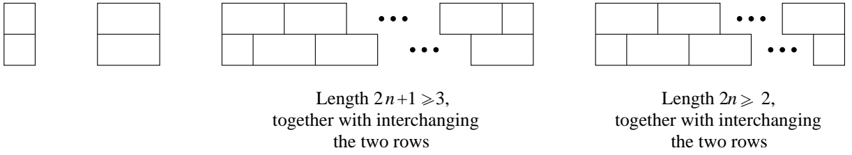
Figure 4.14: The prime blocks
