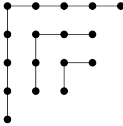
Figure 1.16: The diagonal hooks of the self-conjugate partition 54431
