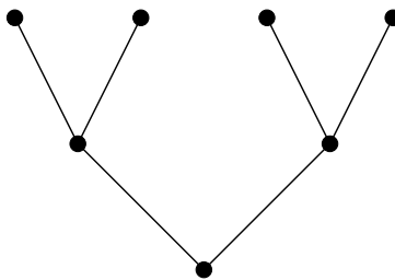
Figure 3.77: The complete dual binary tree P_3
