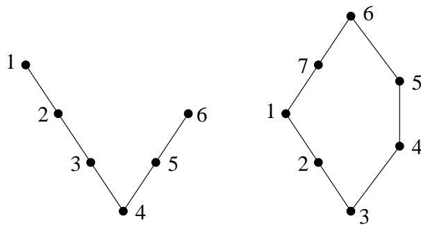
Figure 3.55: Two posets with simple order polynomials
