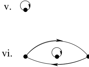
Figure 4.19: Two additional prime graphs
