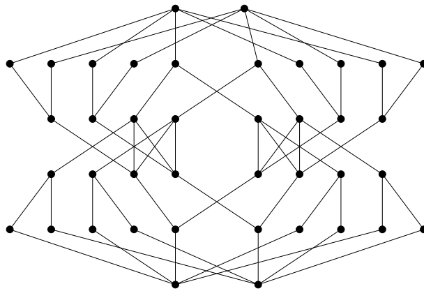
Figure 3.89: A poset Q for which Q \otimes (\mathbf{1} + \mathbf{1}) \cup \{\hat{0}, \hat{1}\} has a nonpositive flag h -vector
