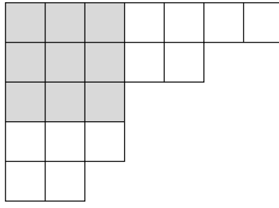
Figure 1.18: The Durfee square of the partition 75332
