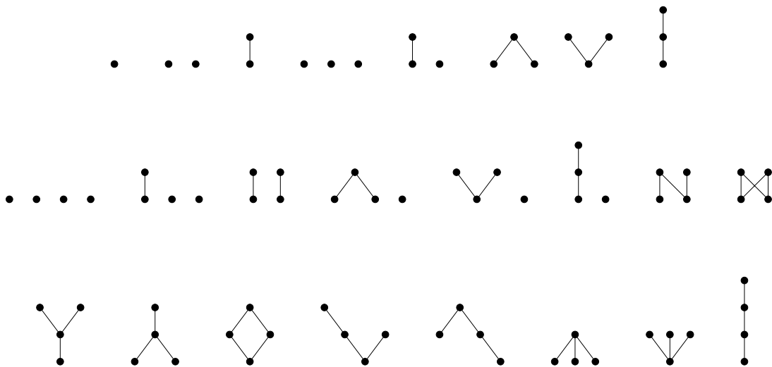
Figure 3.1: The posets with at most four elements
