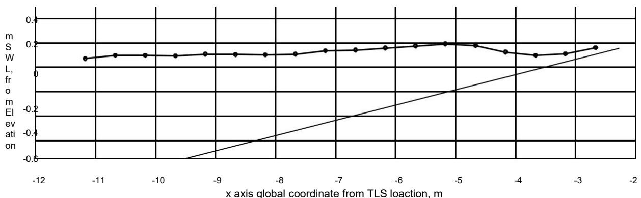
Figure 4 Maximum wave crest profile for Run 2 (dash line and circle) and beach slope (solid line)
