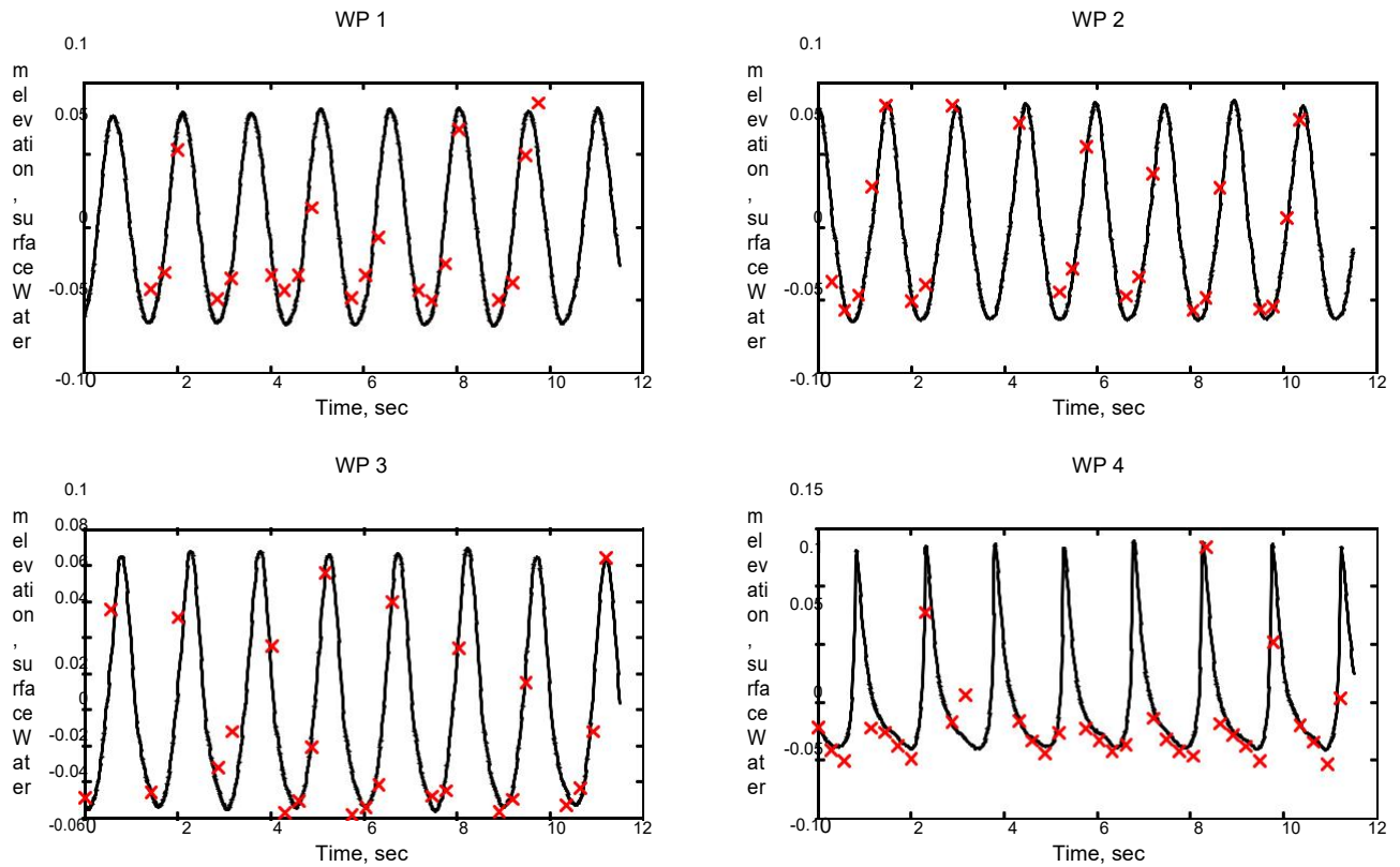
Figure 2 Comparison between wave probe data (solid line, -) and the corresponding TLS data (crosses, x) for Run 8. the TLS line of sight by a wave probe or interference from the flume walls.
