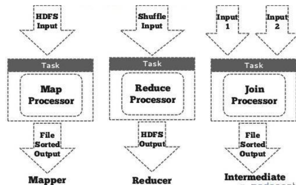
Figure 4. Runtime Tez Model
