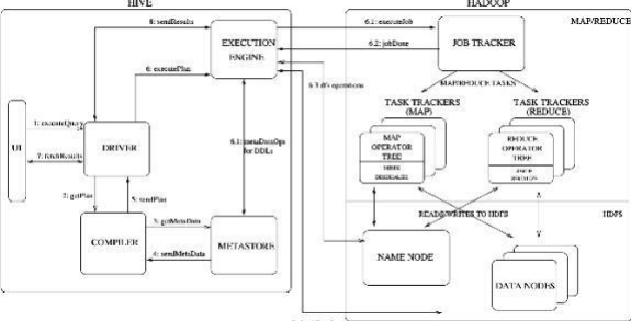
Figure 1. Hadoop eco-system
