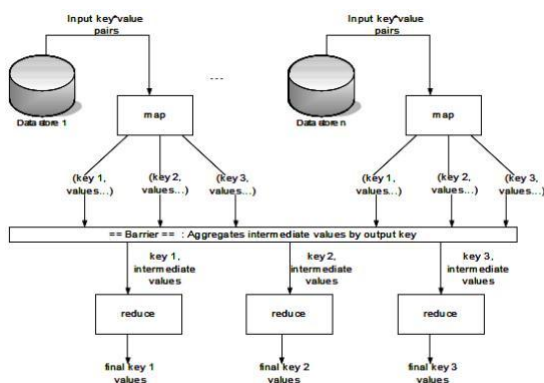
Figure 2. MapReduce Processing
