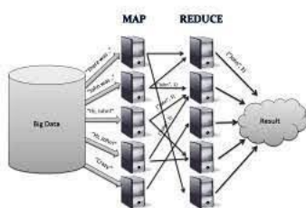
Figure 3. MapReduce Model
